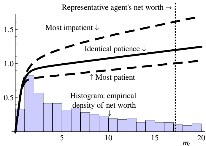
Figure 2 Empirical Wealth Distribution and Consumption Functions of the \beta -Point and \beta -Dist Models
