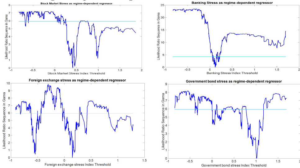
Figure 6: The likelihood ratio for different FSI subcomponent threshold values: The FSI subcomponents as regime-dependent regressors in Advanced Economies, 1994-2013
