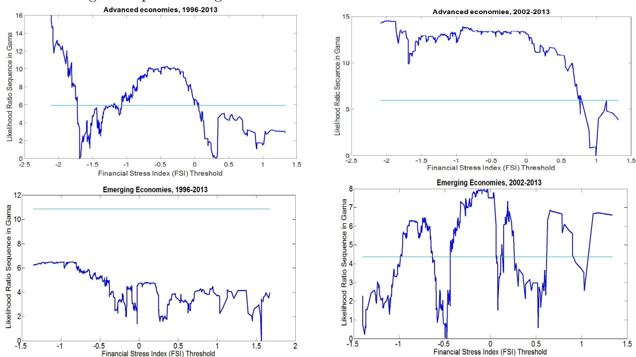
Figure 4: The likelihood ratio for different FSI threshold values: The FSI as threshold variable and regime-dependent regressor
